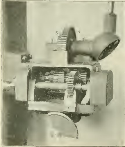
LOWER GEAR BOX. CINCINNATI MILLING MACHINE COMPANY.
